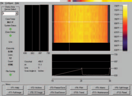
SpotMaster Software for Scan IR II systems
